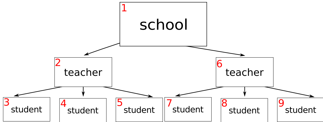
Figure 4. Topological sort is accomplished by depth-first search (Tarjan, 1976) in the opposite direction of the arrows starting from each of the lowest level units (students in this example). Units are assigned a location (the number in the upper left) as soon as all the units that they depend upon are assigned a location. This algorithm is linear in time with the number of units.
